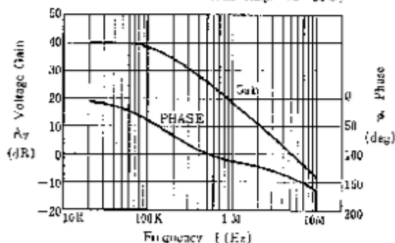
Voltage Gain, Phase vs. Frequency
