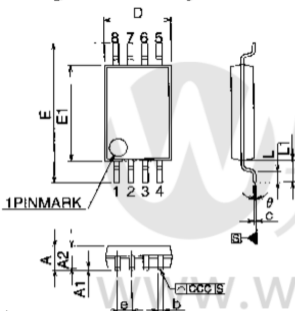
Fig-4 SO8 narrow Package Outline
