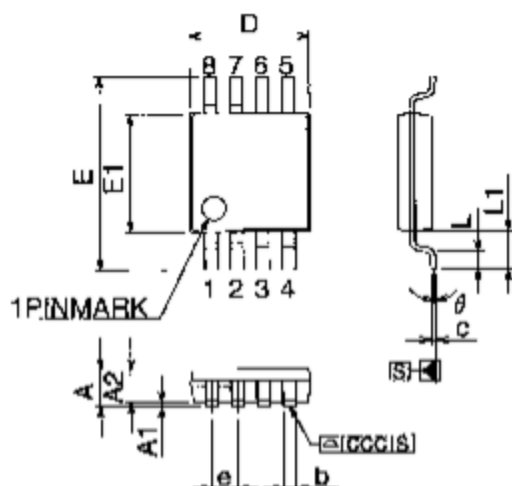
Fig-5 TSSOP Package Outline
