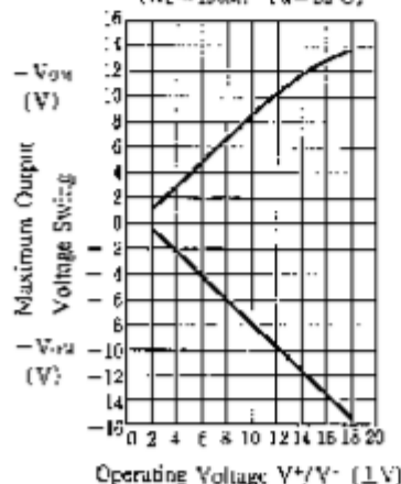
Maximum Output Voltage Swing vs. Operating Voltage
