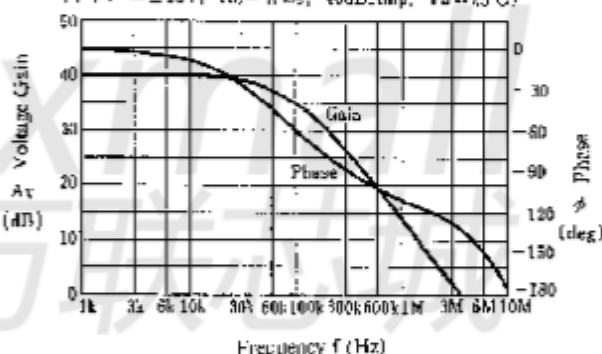
Voltage Gain, Phase Shift vs. Frequency
