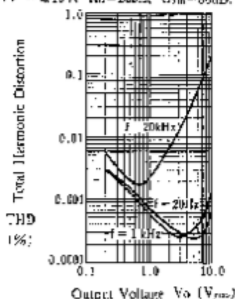
Total Harmonic Distortion vs. Output Voltage
