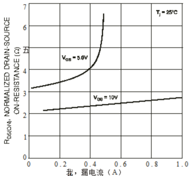
图2导通电阻与漏极电流
