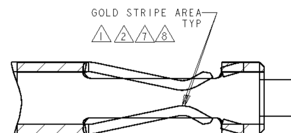
SECTION C-C SCALE 20:1
