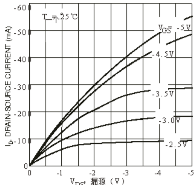
图2漏源电流vs.漏源电压
