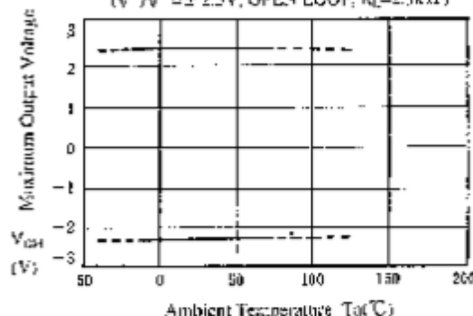
Maximum Output Voltage vs. Temperature
