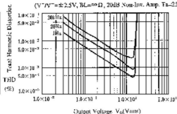
Total Harmonic Distortion vs. Output Voltage
