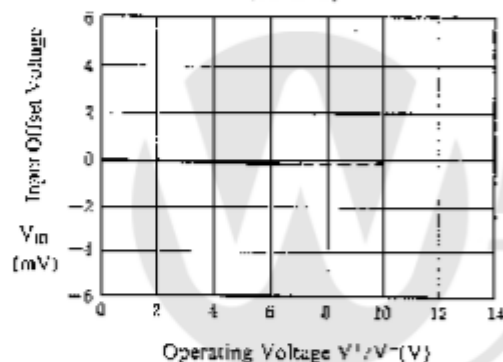
Input Offset Voltage vs. Operating Voltage ( T_a = 25^\circ\text{C} )
