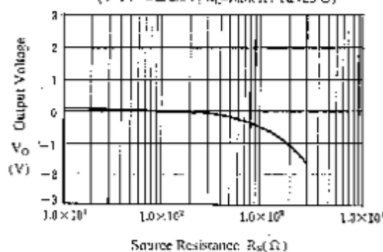
Output Voltage vs. Source Resistance
