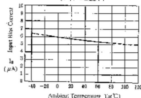
Input Bias Current vs. Temperature ( V^+/V^- = \pm 2.5\text{V} )
