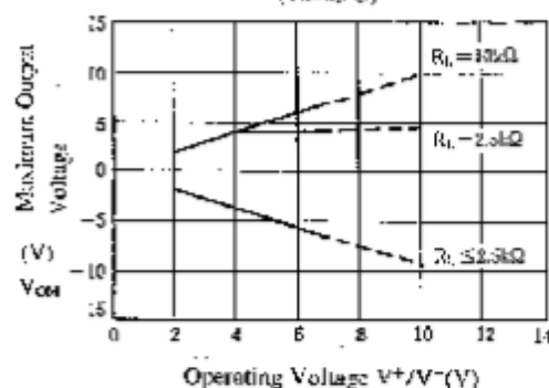
Maximum Output Voltage vs. Operating Voltage, ( T_a = 25^\circ\text{C} )
