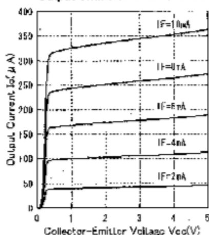
Output Characteristics ( T_a=25^\circ\text{C} )
