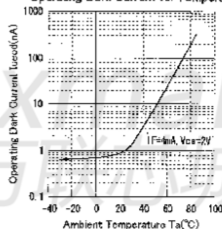
Operating Dark Current vs. Temperature
