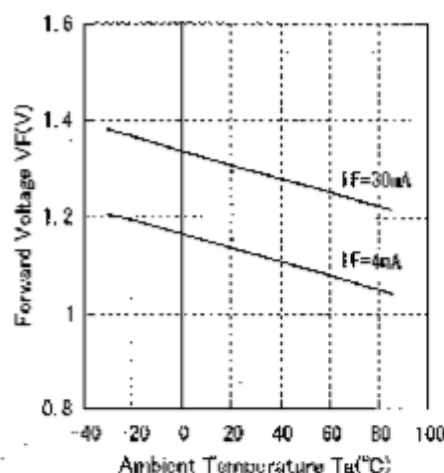
Forward Voltage vs. Temperature
