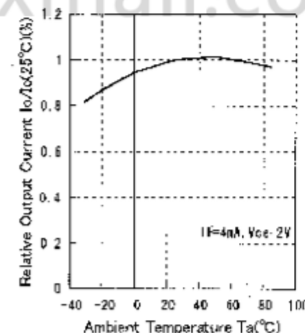
Output Current vs. Temperature
