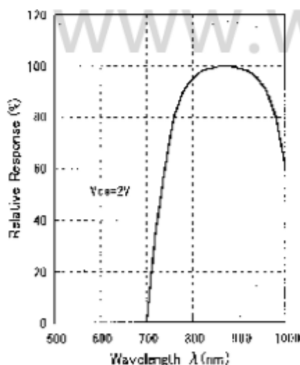
Spectral Response ( T_a=25^\circ\text{C} )
