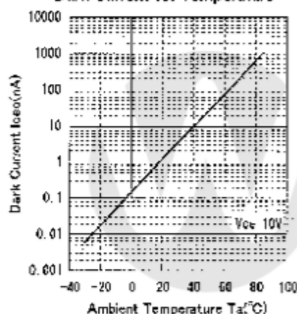
Dark Current vs. Temperature
