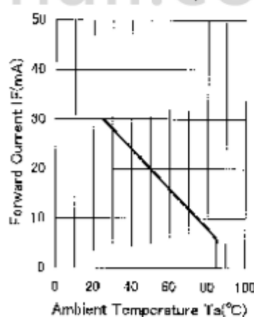
Forward Current vs. Temperature
