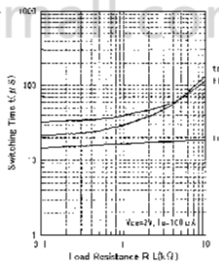
Switching Time vs. Load Resistance ( T_a=25^\circ\text{C} )
