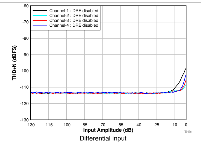
Figure 6. THD+N vs Input Amplitude With DRE Disabled
