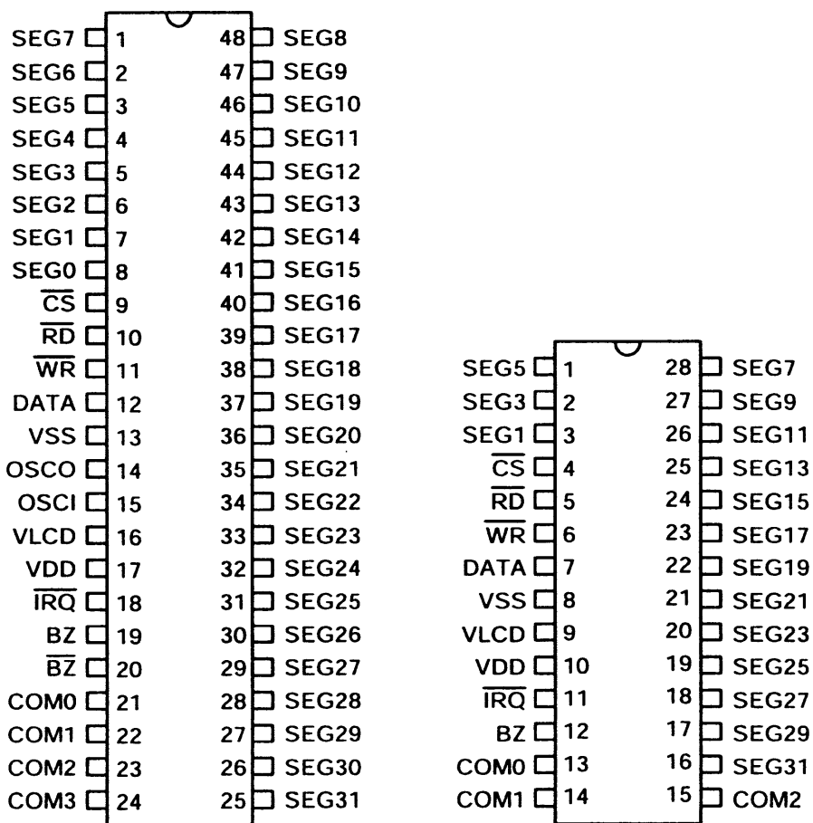
48 SSOP/PDIP
