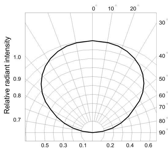
Fig.6 Radiation diagram
