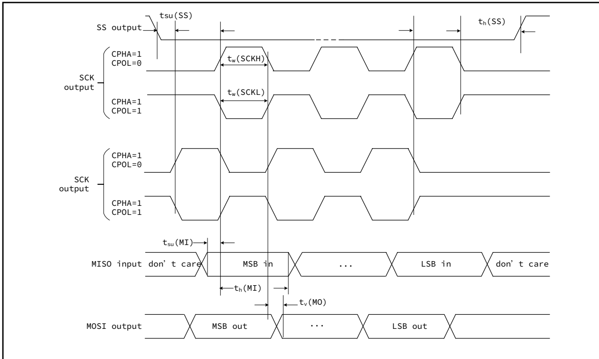
图 3-12 SPI timing diagram -master mode
