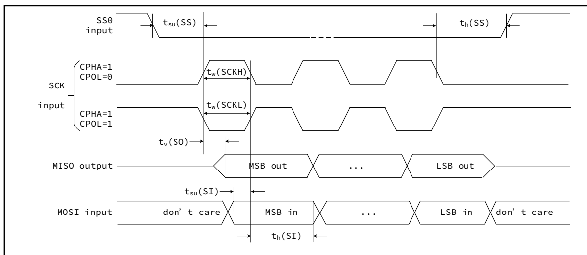
图 3-11 SPI timing diagram -slave mode and CPHA=1
