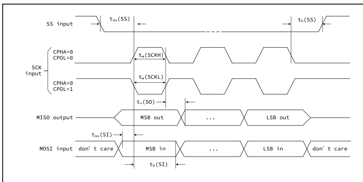
图 3-10 SPI timing diagram -slave mode and CPHA=0
