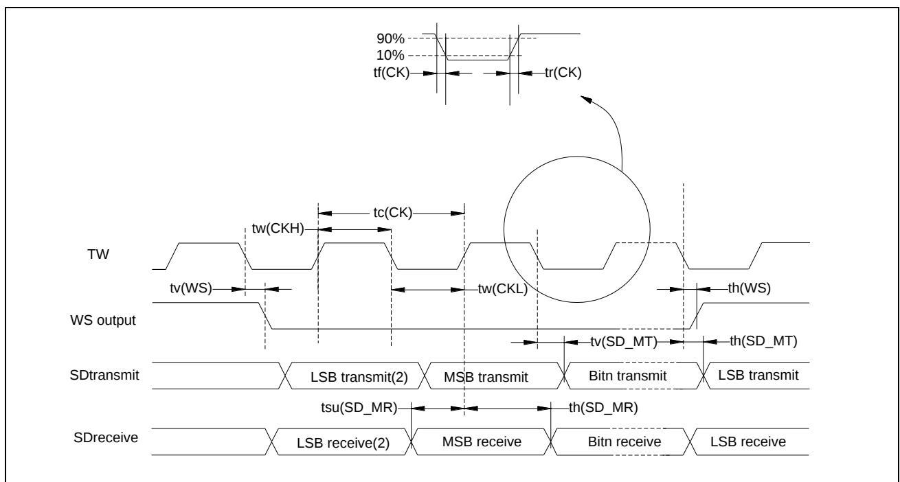
图 7-7 I2S slave timing diagram
