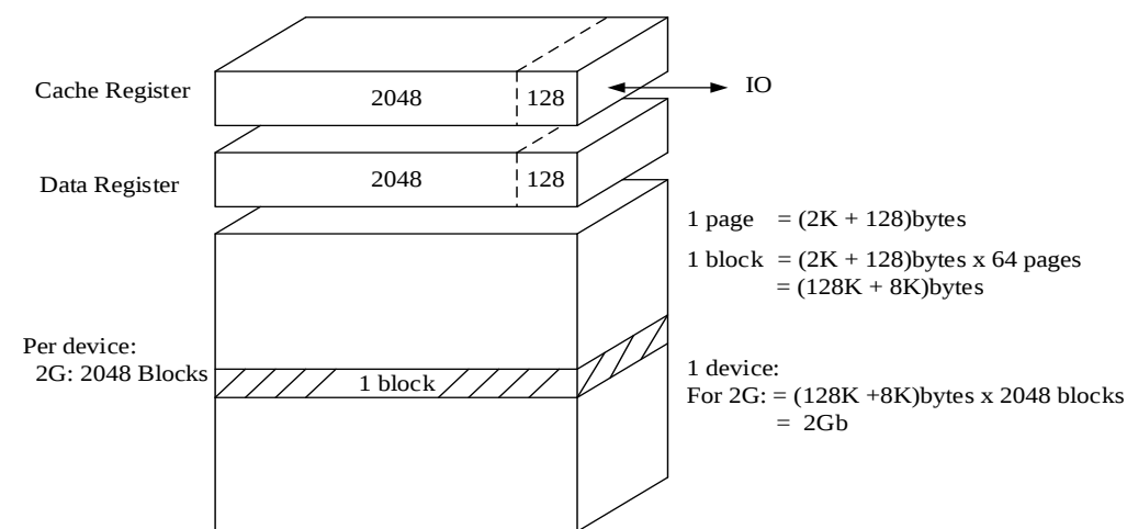
Figure 4. Array Organization
