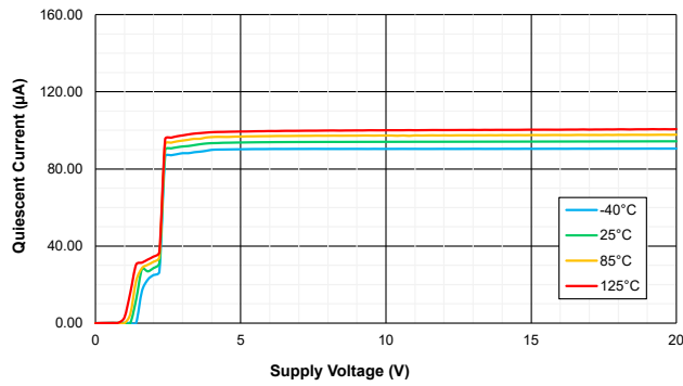
Figure 1. Quiescent Current vs Supply Voltage
