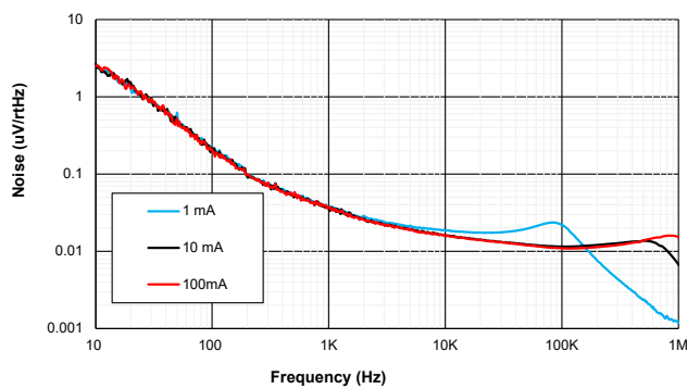
Figure 21. Noise
