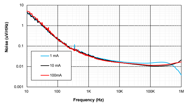
Figure 22. Noise
