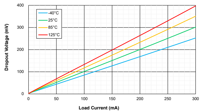
Figure 4. Dropout Voltage vs Load Current
