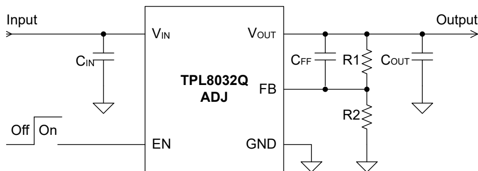
Figure 38. Typical Application Circuit
