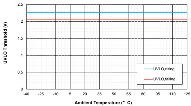
Figure 13. UVLO
