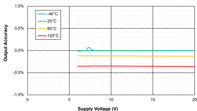
Figure 8. Line Regulation
