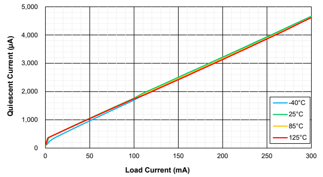
Figure 2. Quiescent Current vs Load Current
