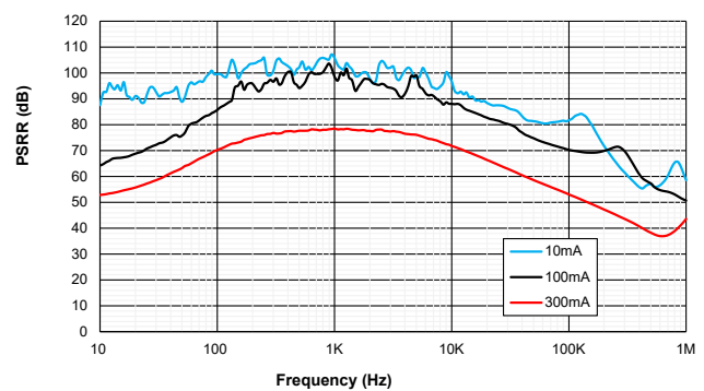
Figure 16. PSRR
