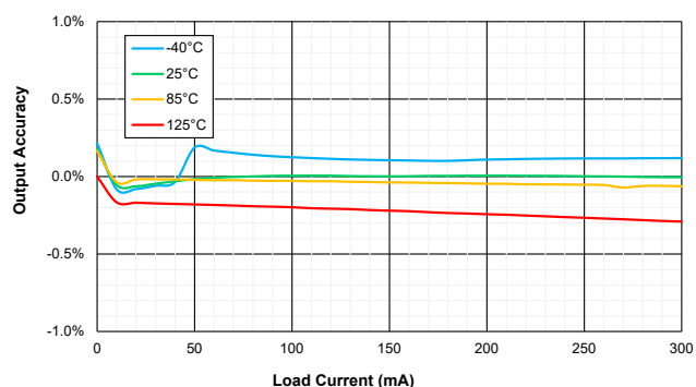
Figure 9. Load Regulation
