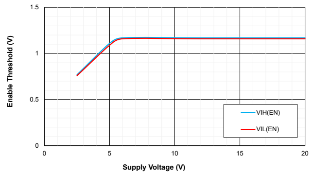
Figure 14. EN Threshold
