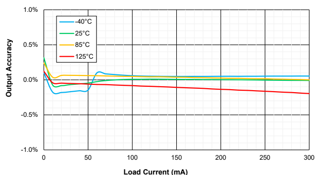
Figure 10. Load Regulation
