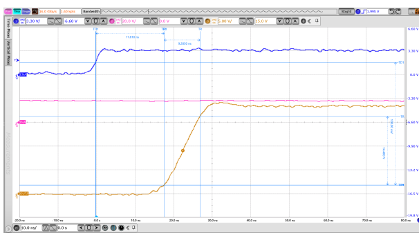
Figure 13. Channel A Rising Edge by ENA
