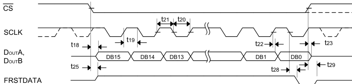
Figure 5. Serial Read Operation (Channel 1)
