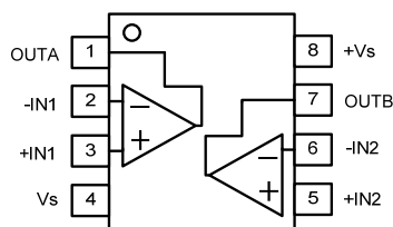
SGM722 SOP-8/MSOP-8/TSSOP-8
