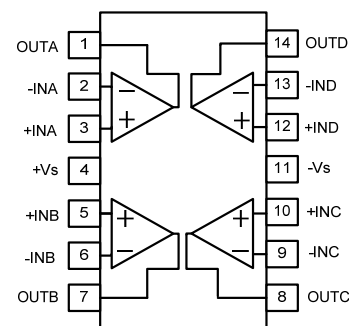
SGM724 SOP-14/TSSOP-14
