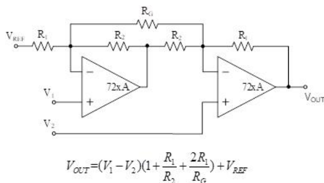
Fig. 17 Instrumentation Amplifier
