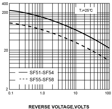
FIG. 5-TYPICAL JUNCTION CAPACITANCE
