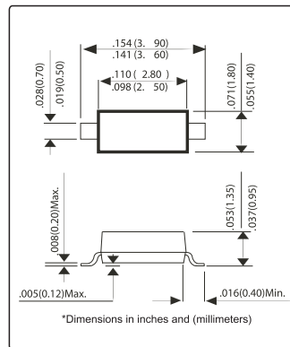
SOD-123
