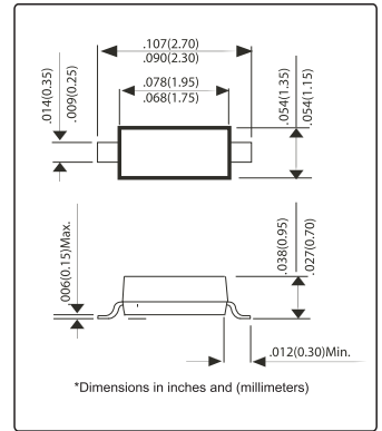
SOD-323
