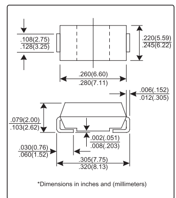
SMC(DO-214AB)
