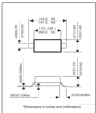
SOD-123FL
