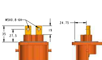
Busbar Type 1
