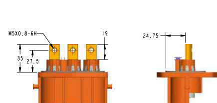
Busbar Type 1
