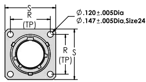
00: Wall Mounting Receptacle 墙装式插座
