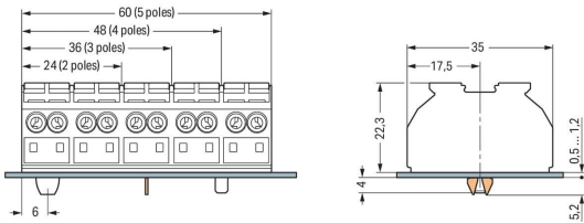
Dimensions in mm Dimensions in mm for chassis-mount terminal strips
