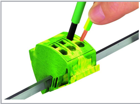
Conductor termination (16 mm 2 /6 AWG):
