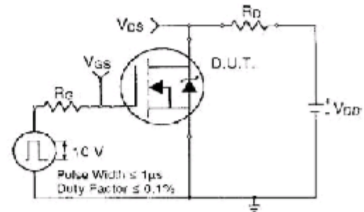
Fig 10a. Switching Time Test Circuit
