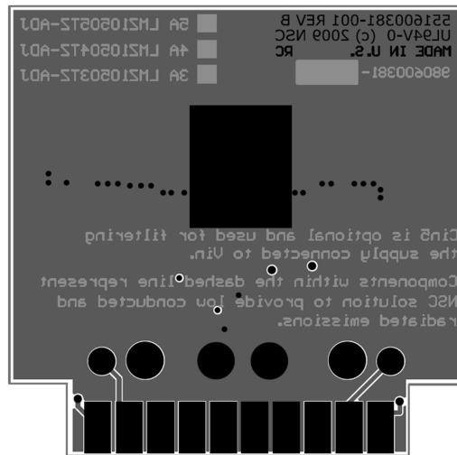
Figure 29. Bottom Copper
