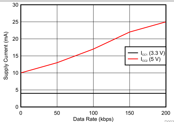
Figure 2. ISO3080 Supply Current vs Data Rate With No Load
