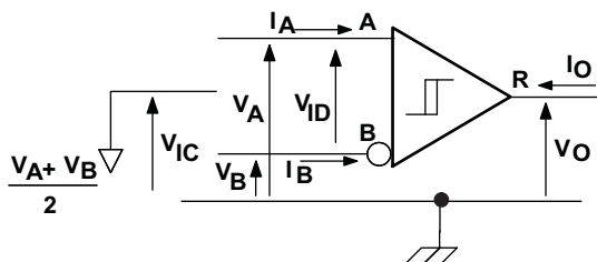
Figure 16. Receiver Voltage and Current Definitions
