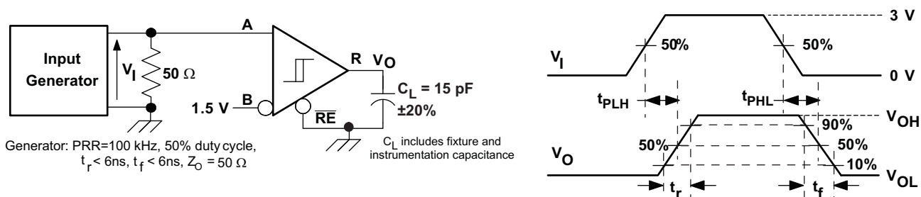
Figure 17. Receiver Switching Test Circuit and Waveforms
