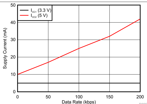
Figure 4. ISO3082 Supply Current vs Data Rate With No Load
