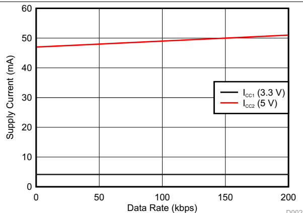
Figure 1. ISO3080 Supply Current vs Data Rate With Load
