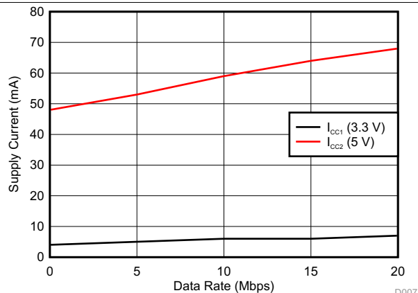
Figure 5. ISO3086 Supply Current vs Data Rate With Load
