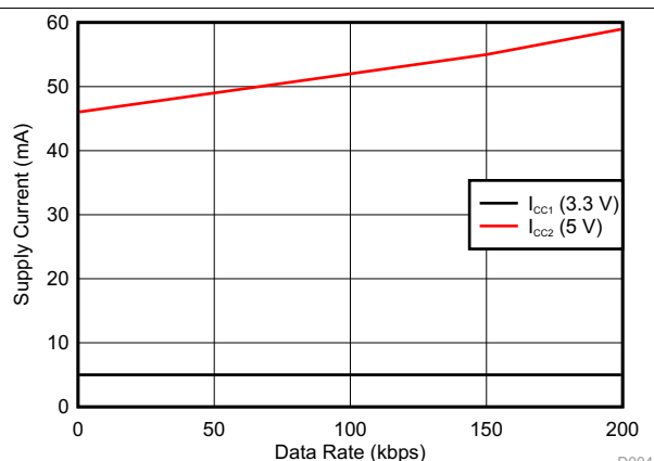
Figure 3. ISO3082 Supply Current vs Data Rate With Load
