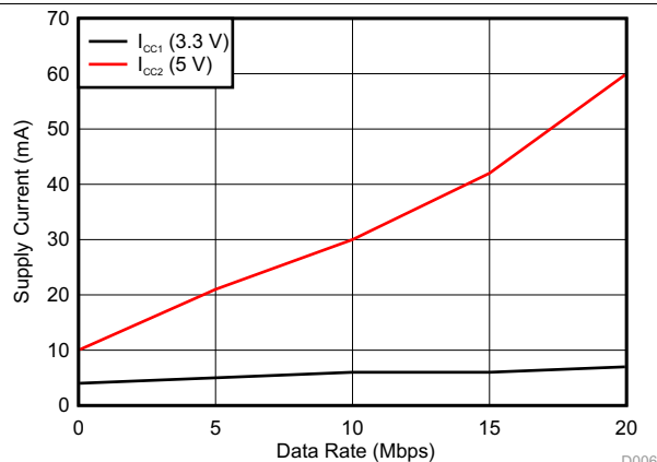
Figure 6. ISO3086 Supply Current vs Data Rate With No Load
