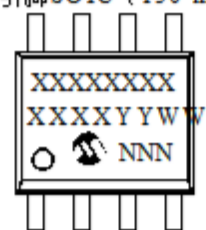
8引脚SOIC (150 mil)
