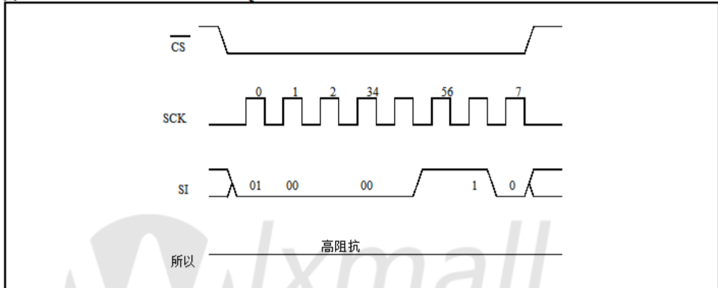
图 3-4: WRITE ENABLE SEQUENCE
